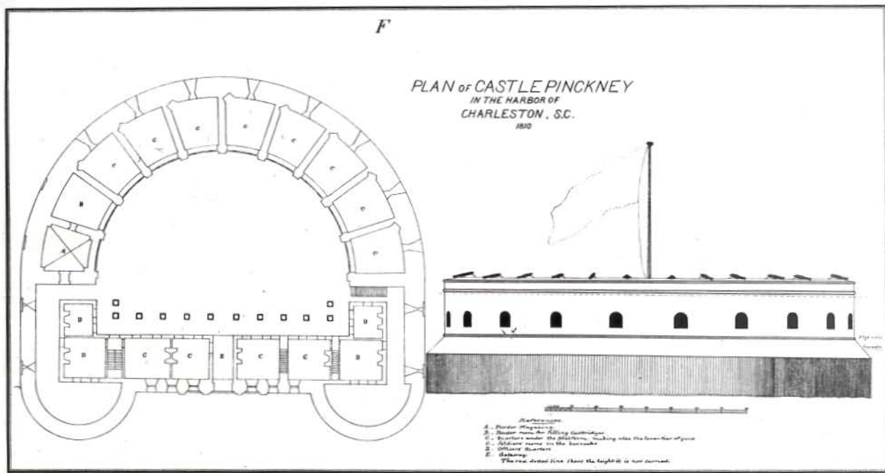
FIGURE 10. United States Department Plan of Castle Pinckney, as constructed in 1808-10. Note the front elevation with tide lines, the floor plan, and room function at the fort.
