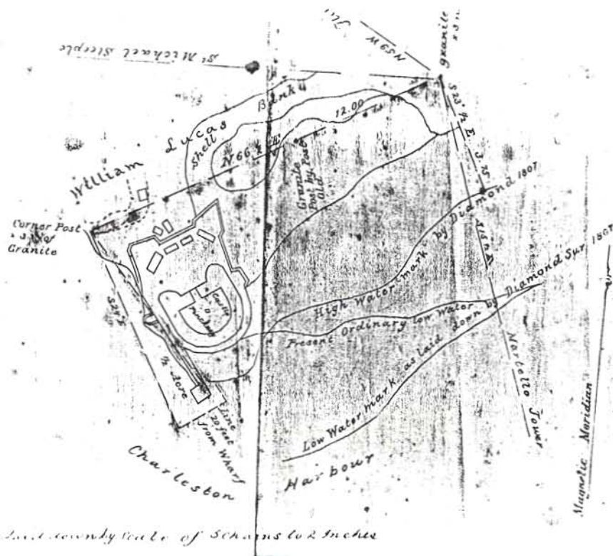
FIGURE 11. Unidentified plat of Castle Pinckney showing palisade wall and buildings located to the rear of the Fort.
